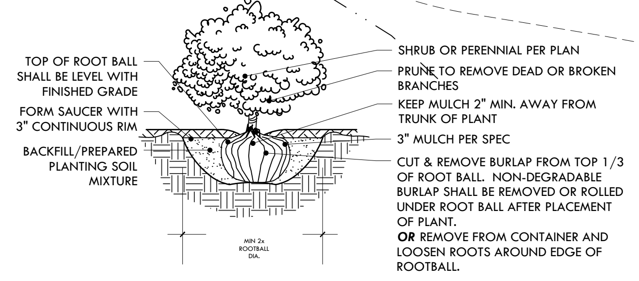
2 SHRUB B&B PLANTING NO SCALE
