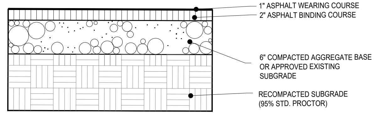
3 BITUMINOUS CONCRETE NO SCALE
