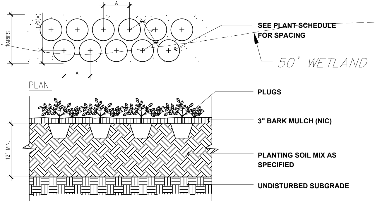
4 PERENNIAL PLUGS NO SCALE
